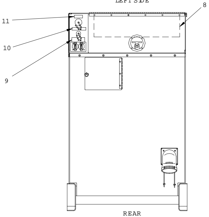
Figure 1. Generator Set, 60KW (Sheet 1 of 2)
