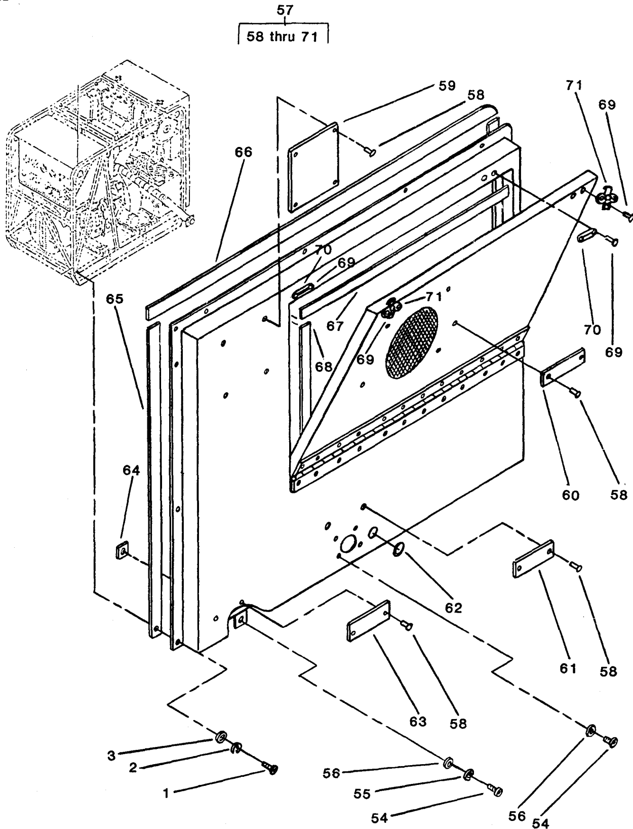
Figure 49, Panels, (3roup 10 (Sheet 5 of 7).
