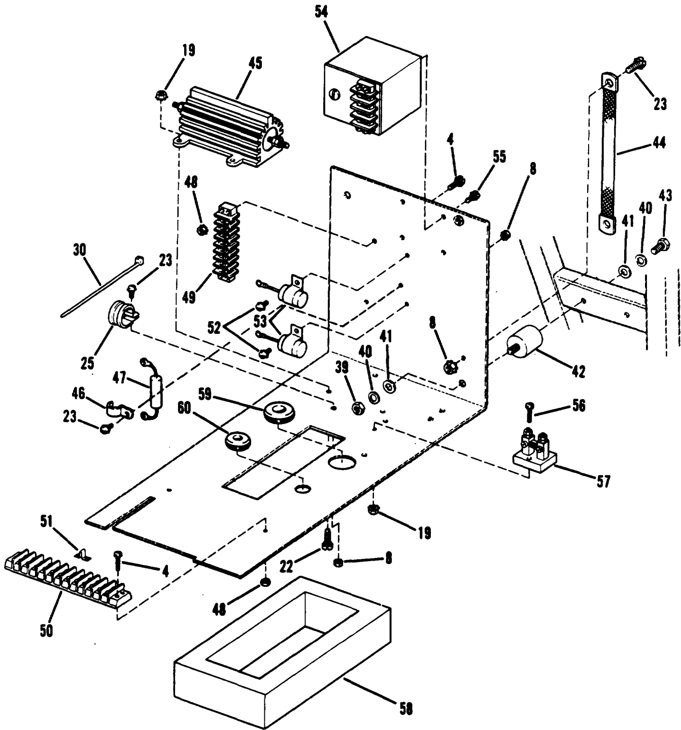
Figure 37. Generator Control Assembly 28 VDC, Group 08 (Generator Controls and Instruments) (Sheet 2 of 3)
