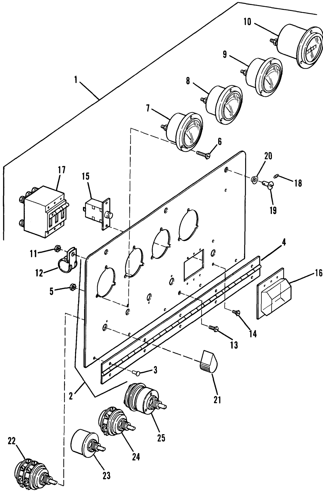
Figure 42. Meter Panel 400 Hz, Group 08 (Generator Controls and instruments)
