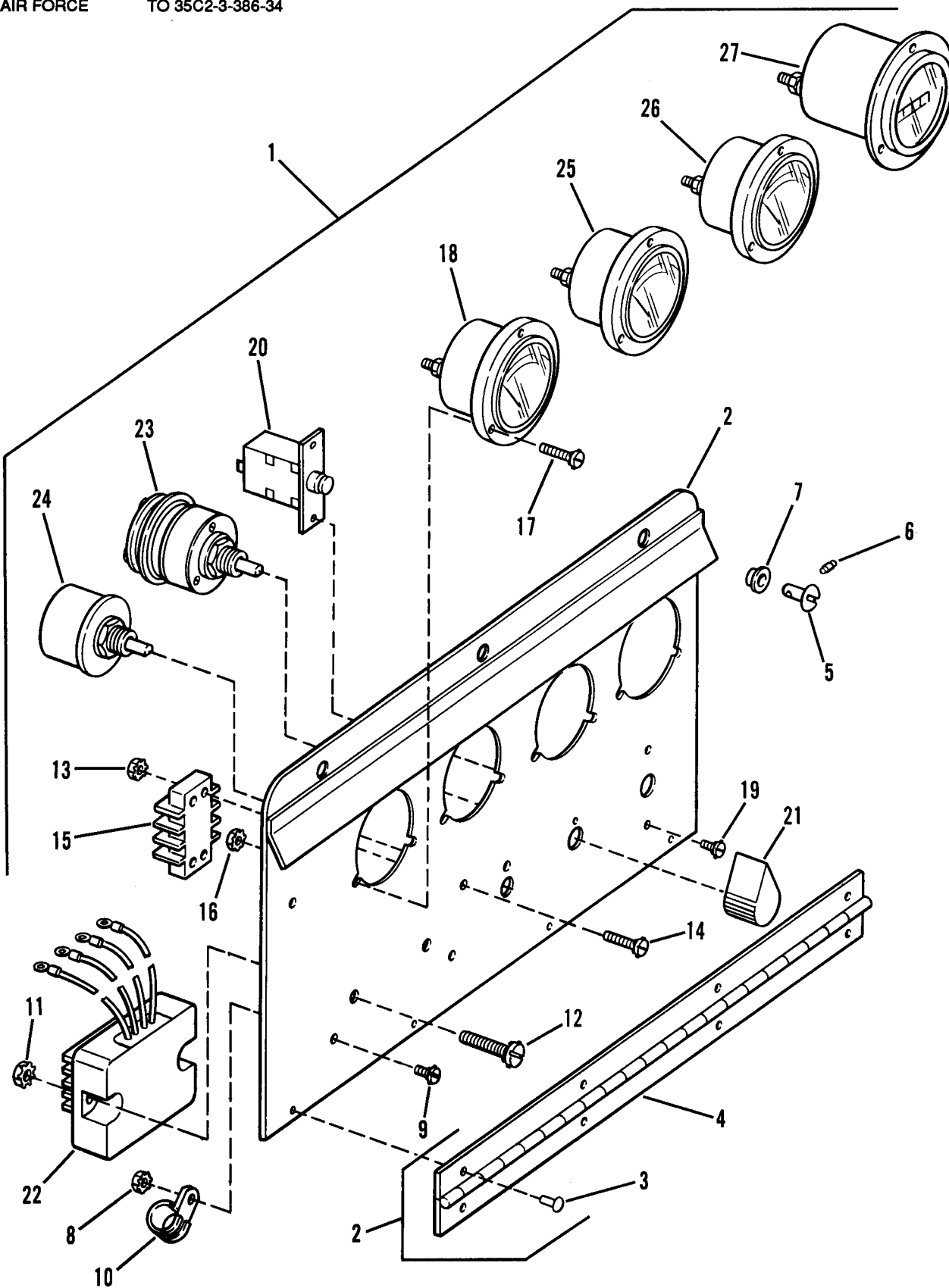
Figure 35. Meter Panel 28 VDC, Group 08 (Generator Controls and Instruments)
