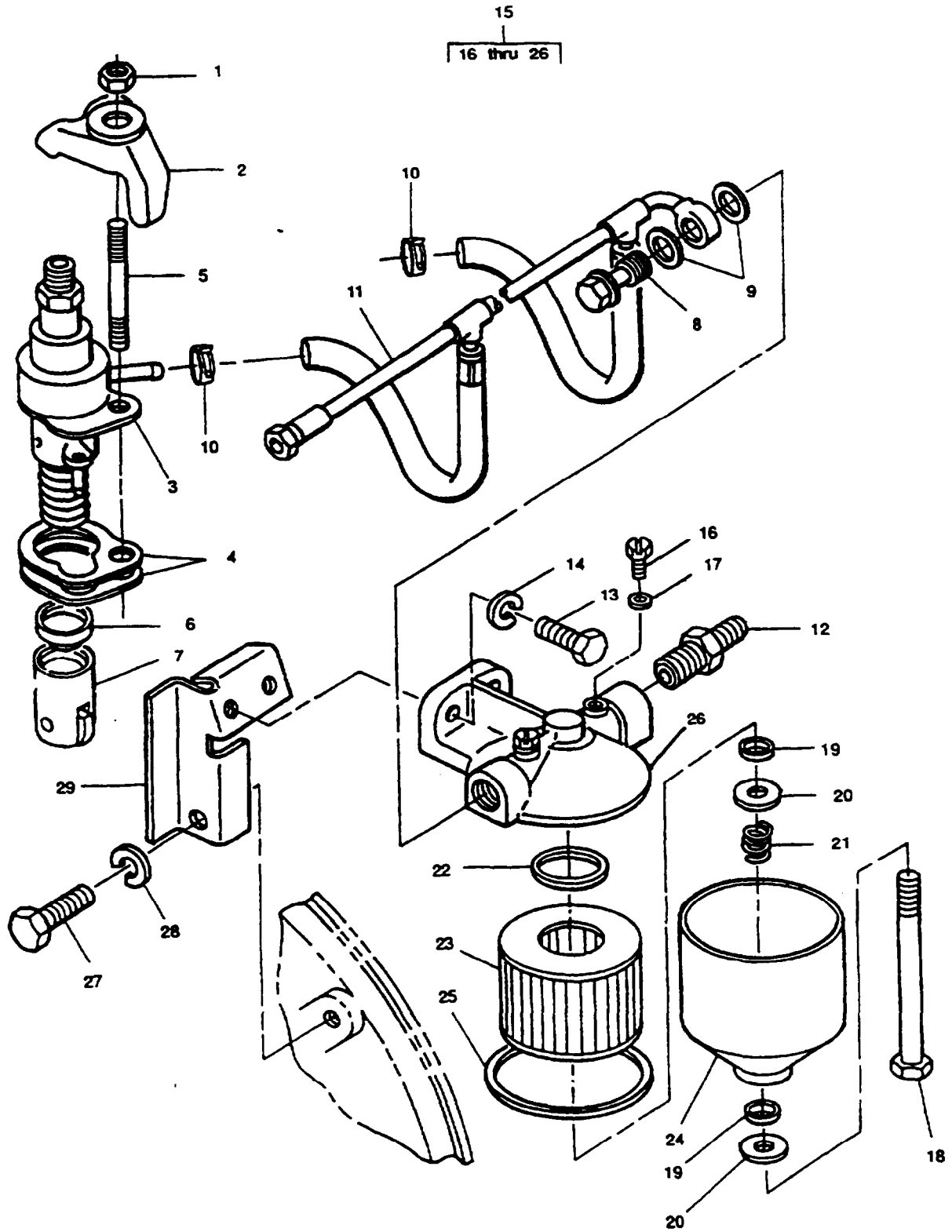
Figure 4. Fuel Pump and Lines
