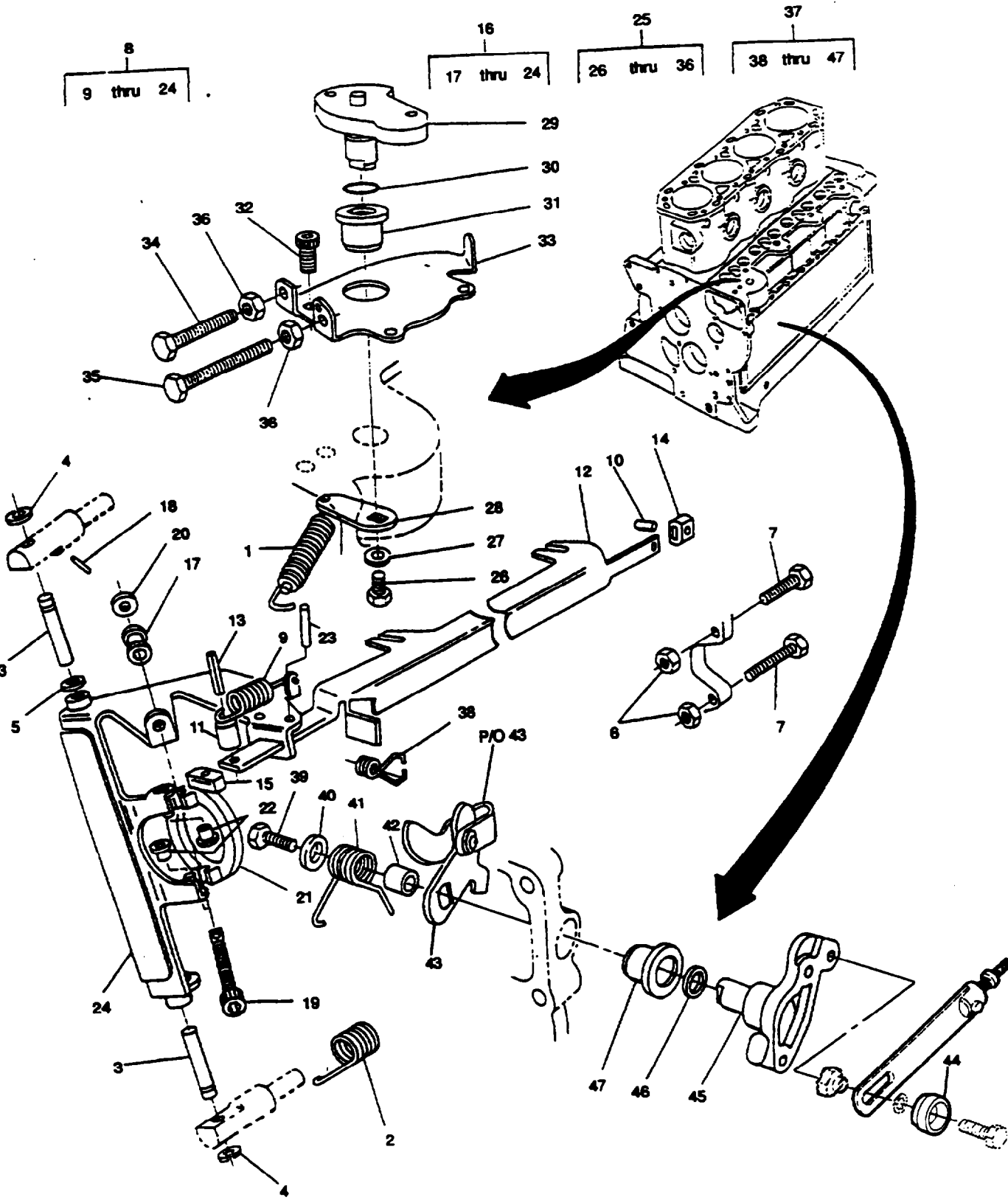
Figure 9. Governor System
