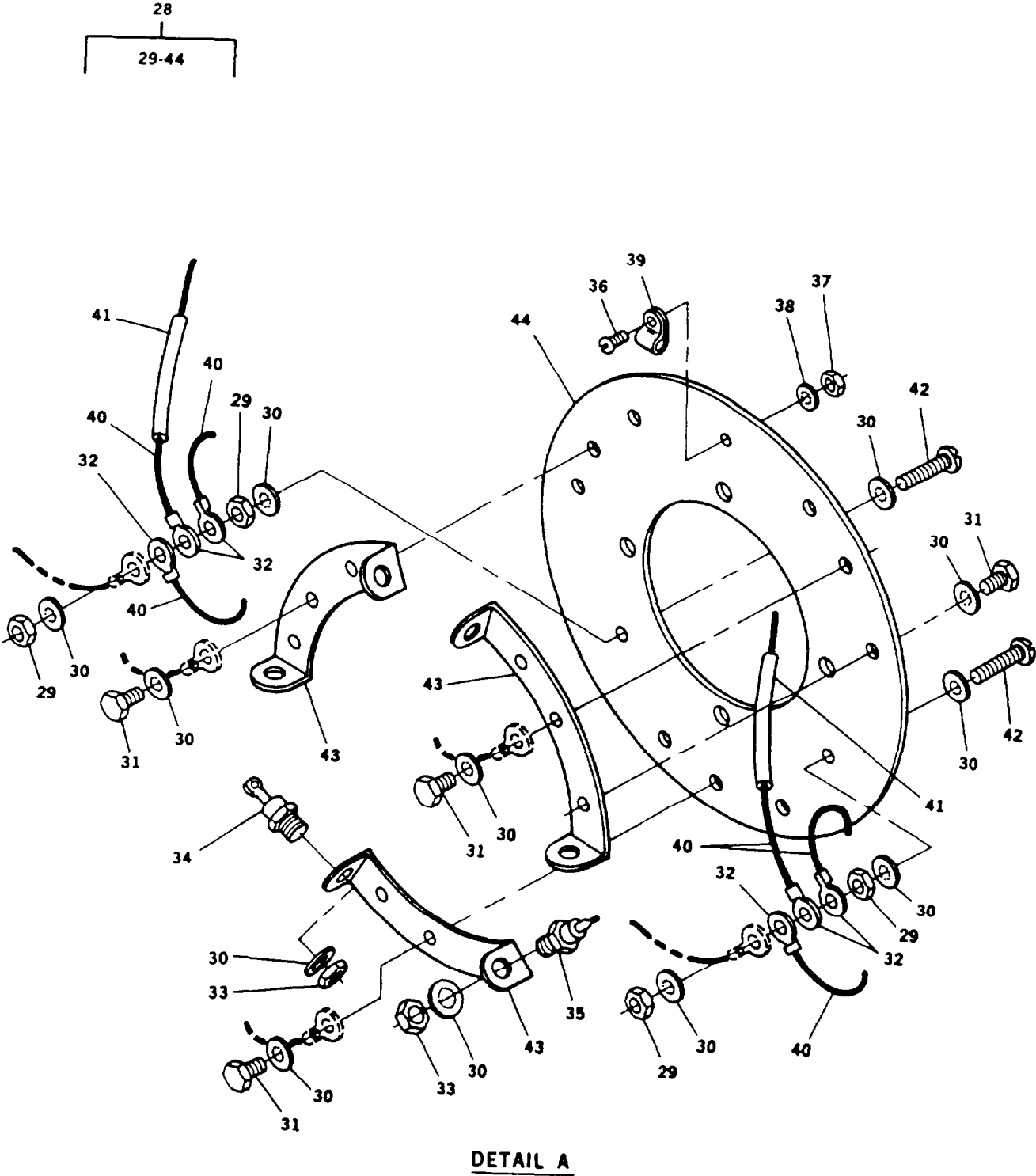
FIGURE 22. Generator Assembly, 50/60 Hz (Sheet 2 of 2)
