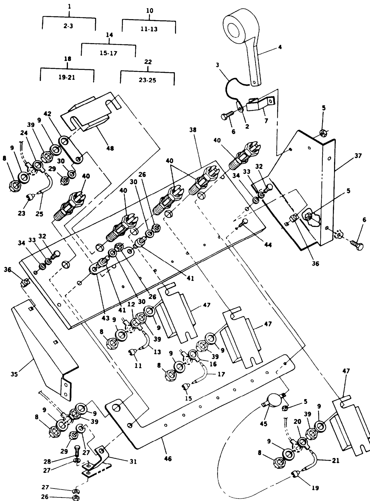
FIGURE 18. Load Terminal Board
